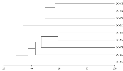
Fig. 5. Dendrogram of similarity of sampling stations and Bidimensional ordination (MDS) of sampling stations (stress = 0.02). LC, Los Cristianos; C, Cymodocea nodosa meadows, M, sandy bare bottoms.
